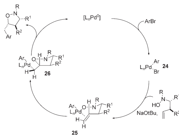
Scheme 1. Catalytic cycle of the Pd-catalyzed carboetherification reaction of N -butenylhydroxylamines.
